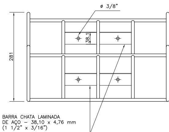
VISTA FRONTAL
